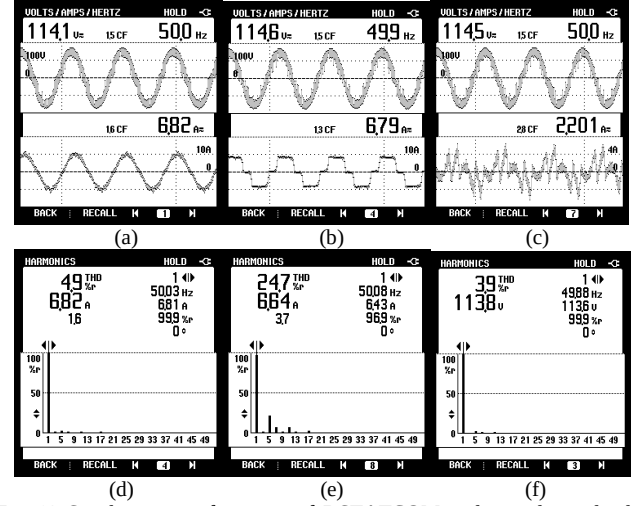
Fig. 12 Steady state performance of DSTATCOM under nonlinear load (a) v_{ab} and i_{sa} (b) v_{ab} and i_{la} (c) v_{ab} and i_{ca} (d) harmonic spectrum of i_{sa} (e) harmonic spectrum of i_{la} and (f) harmonic spectrum of v_{ab} .
