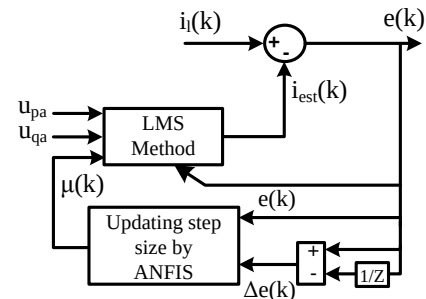
Fig. 2 Error minimization by ANFIS-LMS
