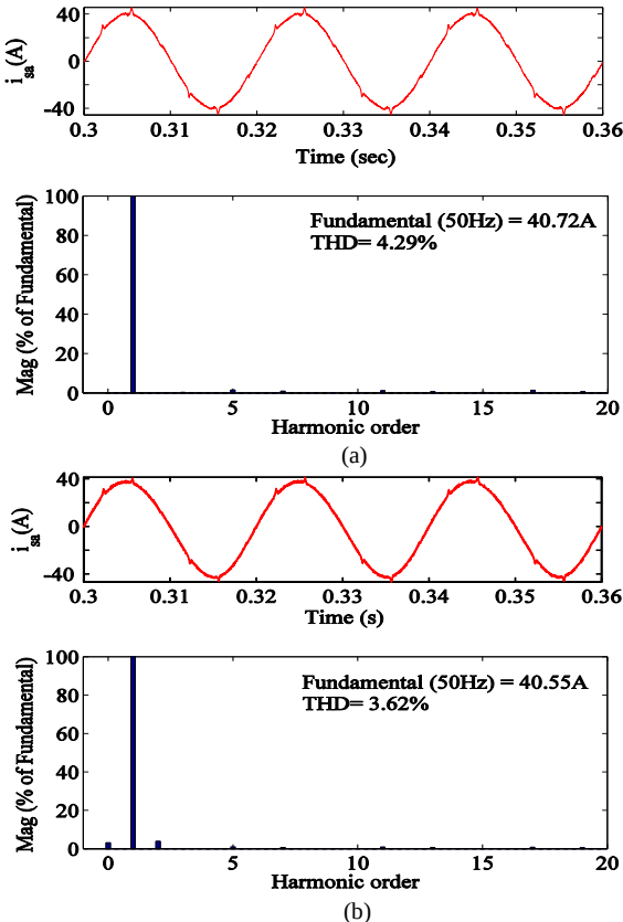
Fig. 10 Harmonic spectra of (a) i_{sa} , For LMS (b) i_{sa} , for VSLMS
