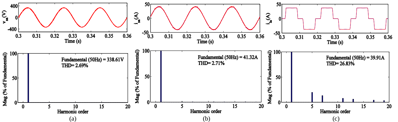
Fig. 8 Waveforms and harmonic spectra of phase ‘a’ of (a) PCC voltage, v_{sa} (b) supply current, i_{sa} and (c) load current, i_{la} in voltage regulation mode
