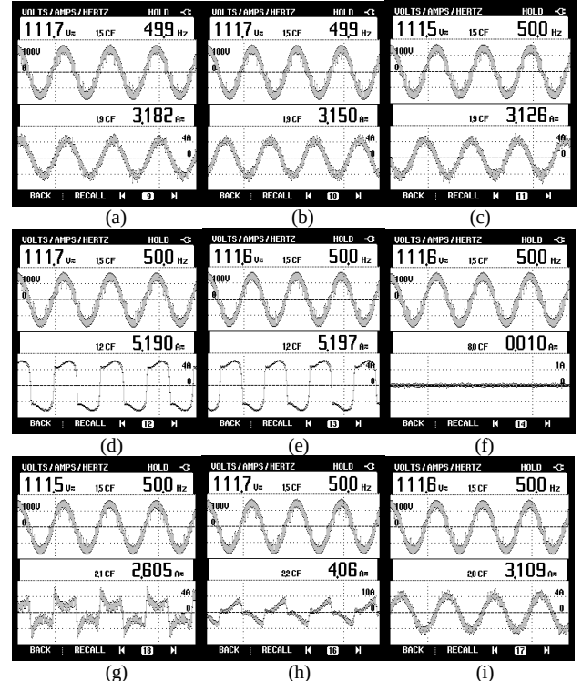
Fig. 13 Load balancing using DSTATCOM with unbalanced nonlinear load (a-c) i_{sa} , i_{sb} , and i_{sc} with v_{ab} (d-f) i_{la} , i_{lb} , and i_{lc} with v_{ab} (g-i) i_{ca} , i_{cb} , and i_{cc} with v_{ab} .
